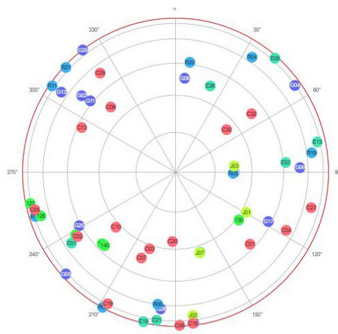
All Constellations
