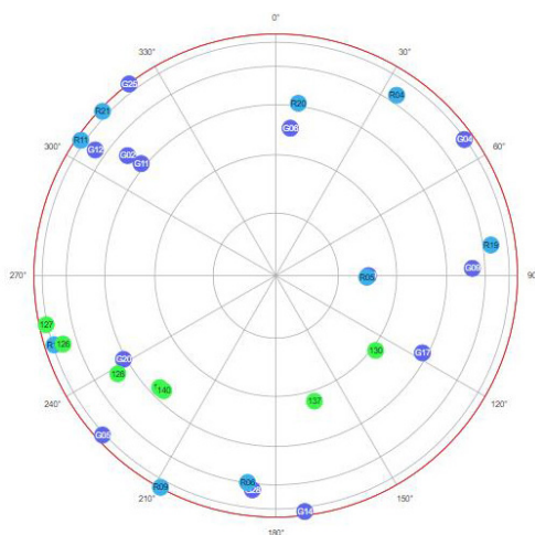
GPS + GLONASS
